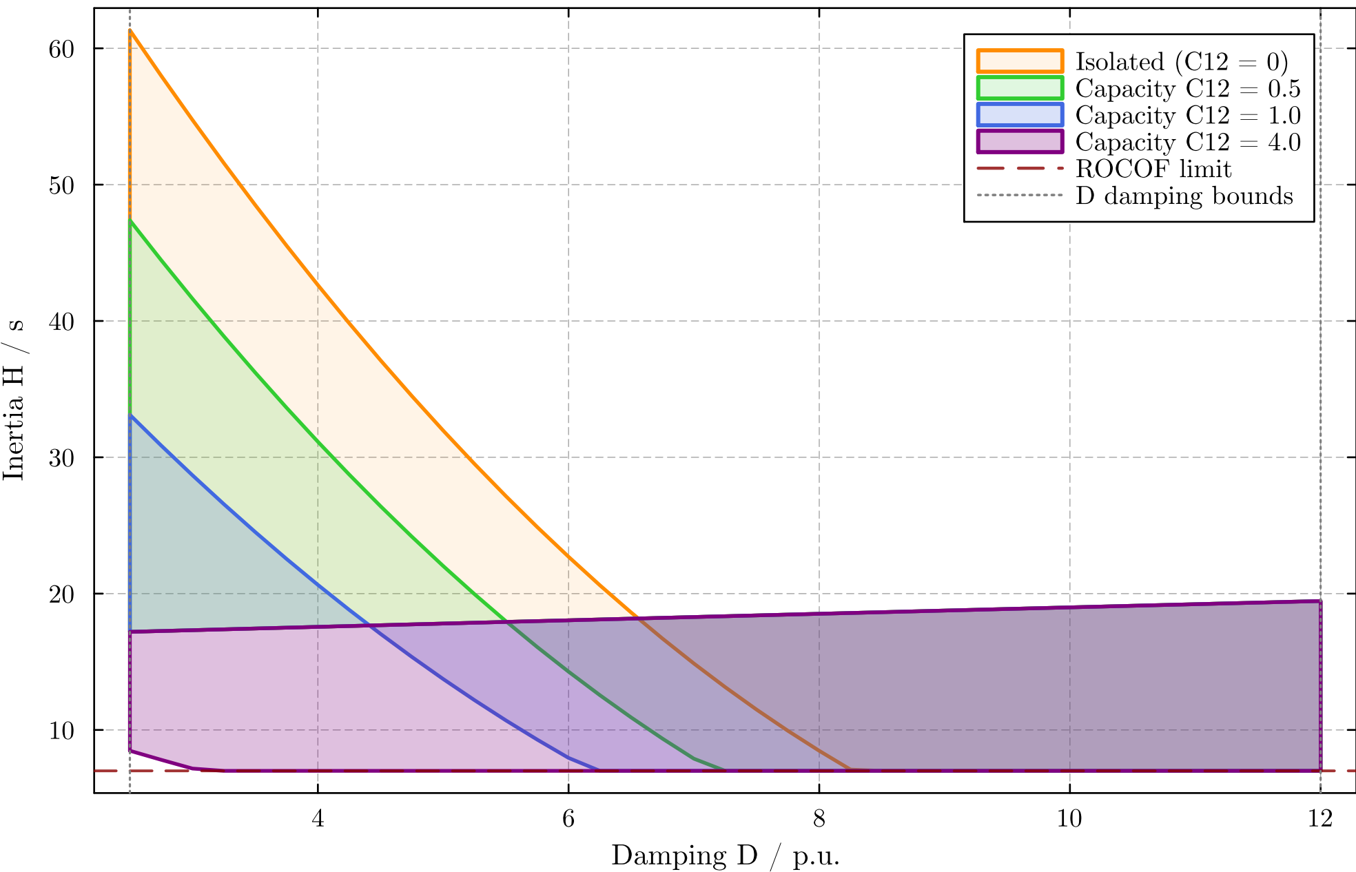
Impact of Tie-line Capacity on Area 1 Security Region
